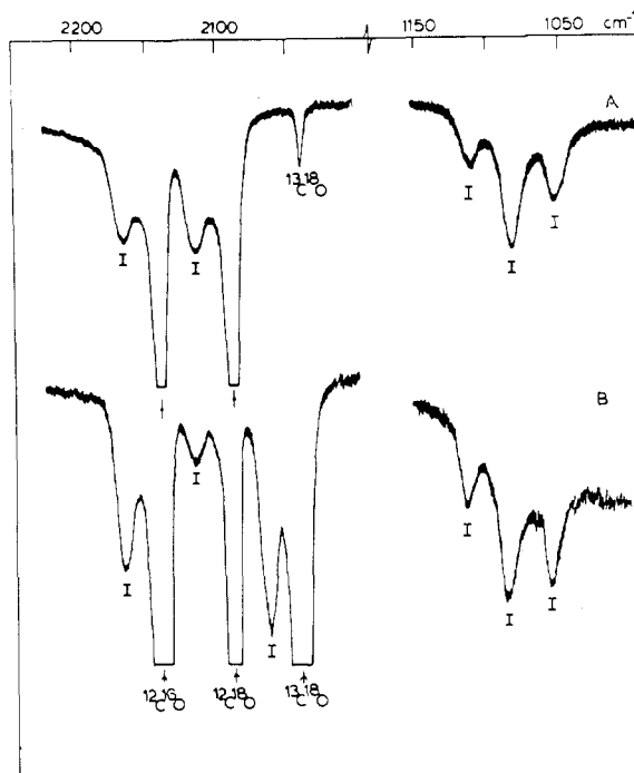
Figure 6. The matrix infrared spectrum of the products formed when Ag atoms are cocondensed with (A) 12 C 16 O: 12 C 18 O: 16 O 2 : 16 O 18 O: 18 O 2 = 1:1:1:2:1 and (B) 12 C 16 O: 13 C 18 O: 16 O 2 : 16 O 18 O: 18 O 2 = 1:1:1:2:1 at 10–12 K showing the characteristic isotopic patterns for an [(OC)Ag] + O 2 - complex (labeled I). (Note that the commercially available 12 C 16 O: 13 C 16 O mixtures contain about 7% of 12 C 18 O: 13 C 16 O as seen in (B).) Taken from ref 26.
